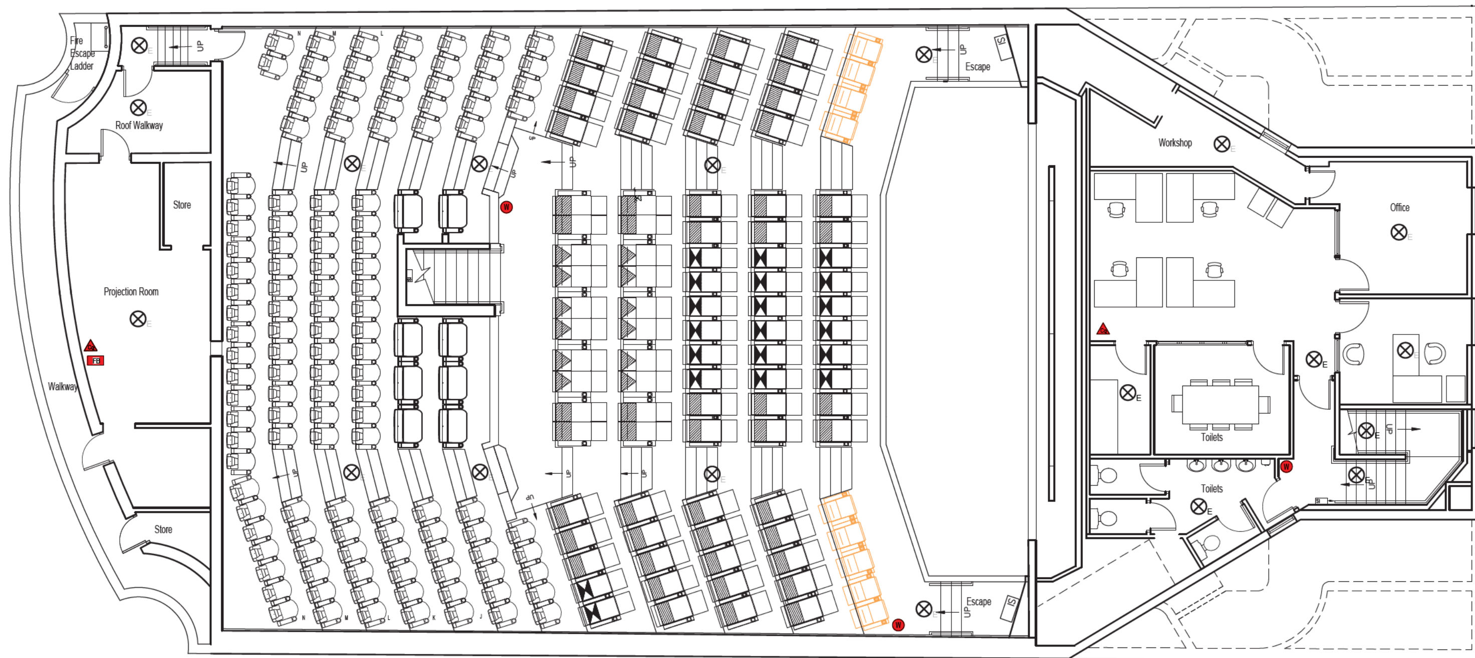
CIRCLE LEVEL PLAN SCALE 1:100@A1
