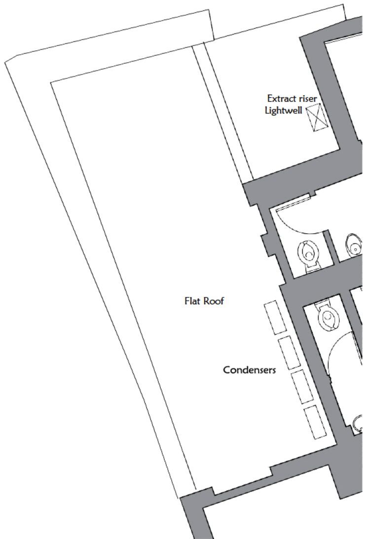
First Floor General Arrangement Scale 1:50
