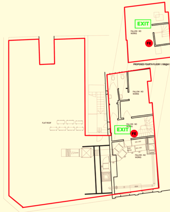
PROPOSED THIRD FLOOR 1:100@A1
